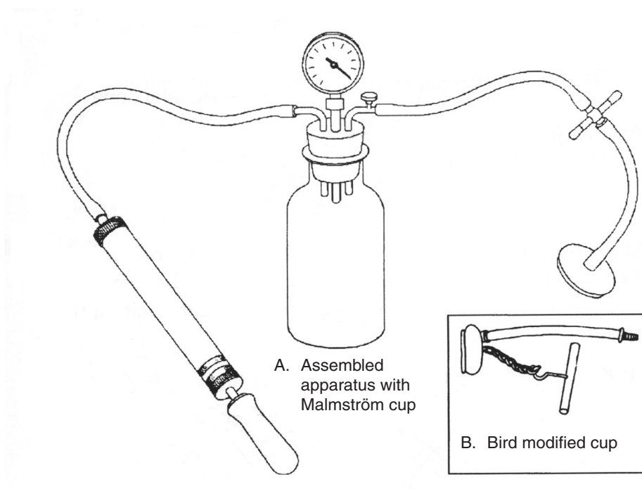
Figure 8.1: Vacuum hand pump
